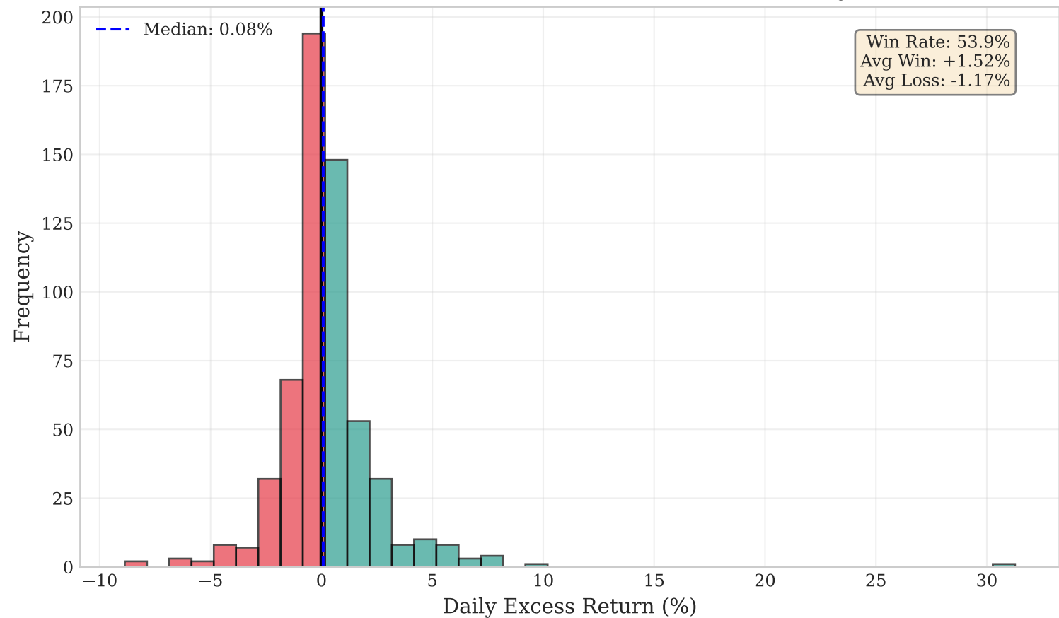
P&L Distribution: LSTM Attention (584 Active Days)
