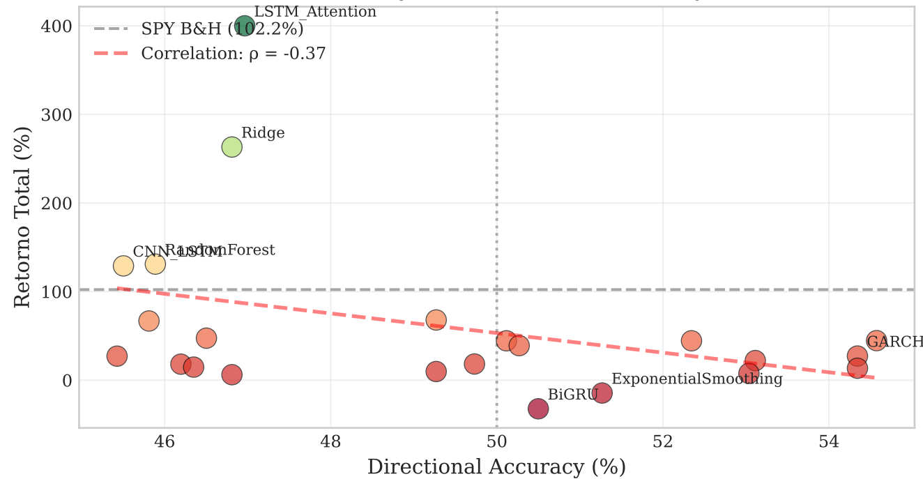
La Paradoja del Directional Accuracy
