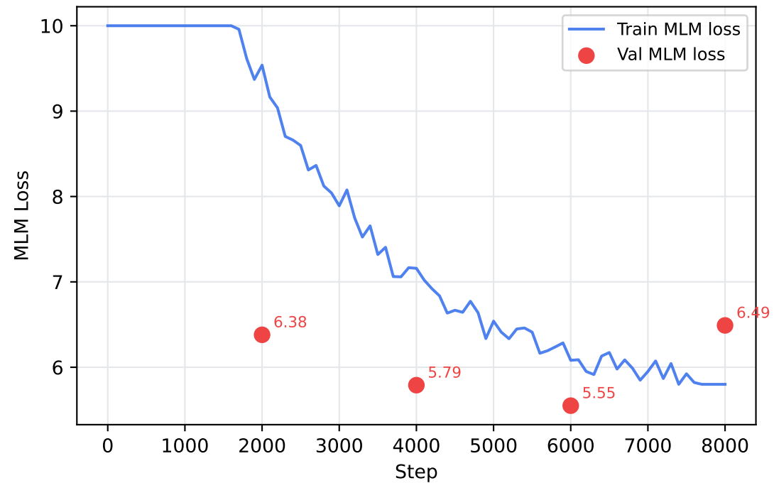
(a) Stage A — MLM Pretraining
