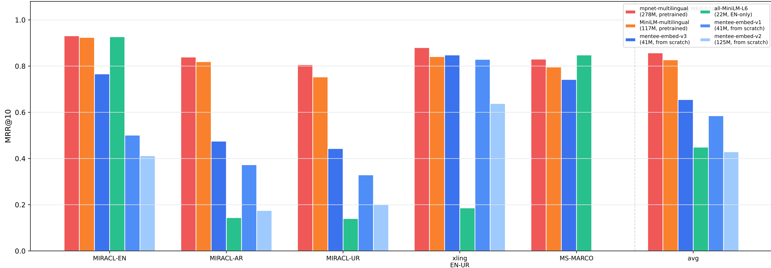
Protocol A — In-batch Retrieval MRR@10 (pool ≈ 97 candidates)
