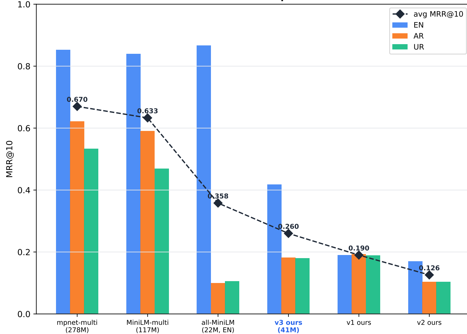
Protocol B — MIRACL Wikipedia Retrieval
