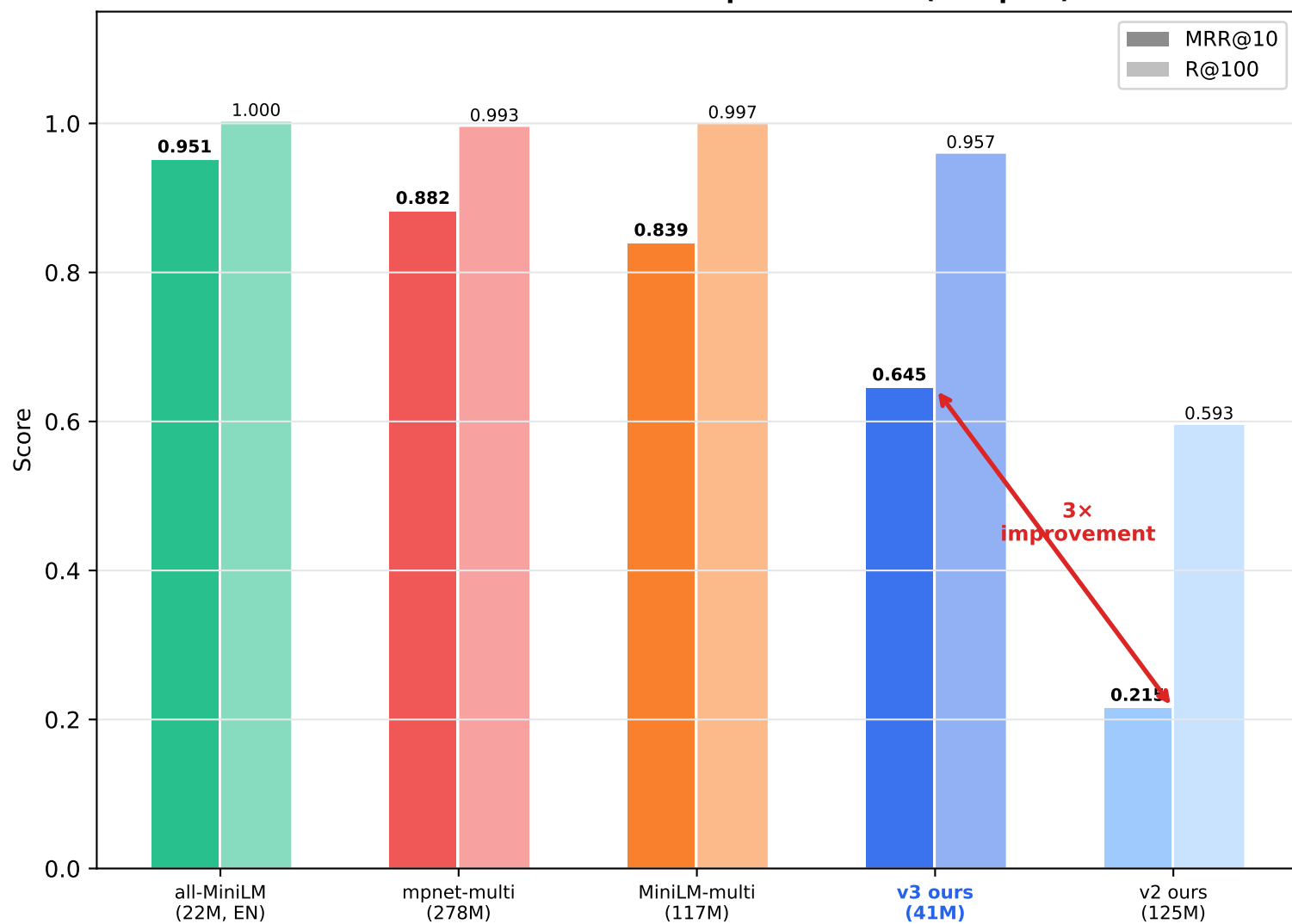
Protocol C — MS-MARCO Corpus Retrieval (10K pool)
