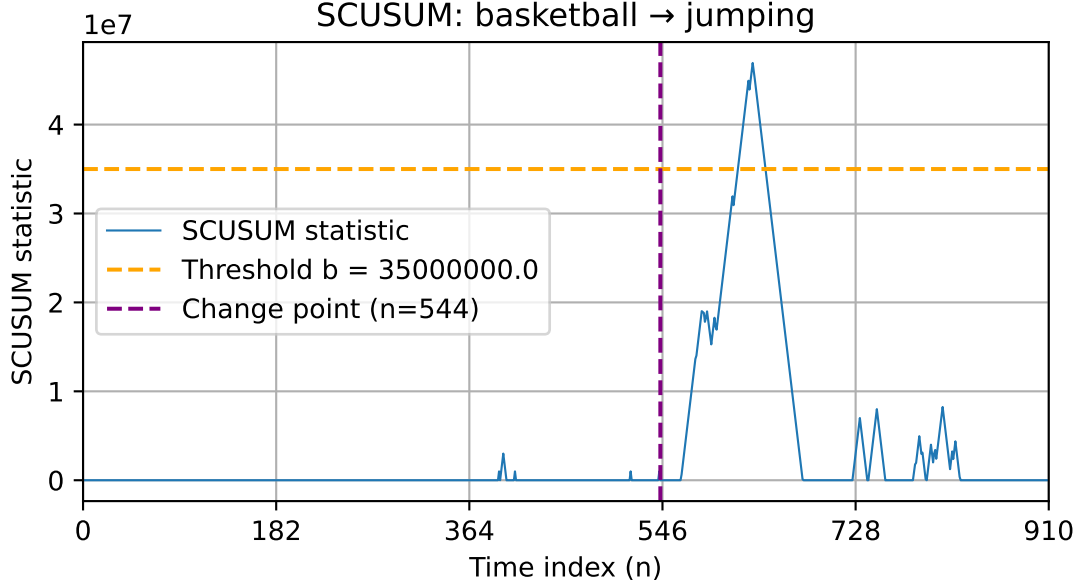
SCUSUM: basketball → jumping
