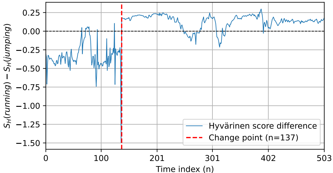
1e8 Hyvärinen Score Difference: running \rightarrow jumping
