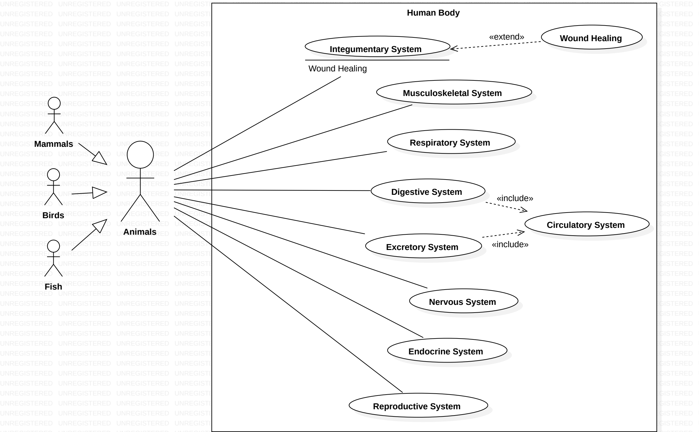
Model2::UseCaseDiagram1
