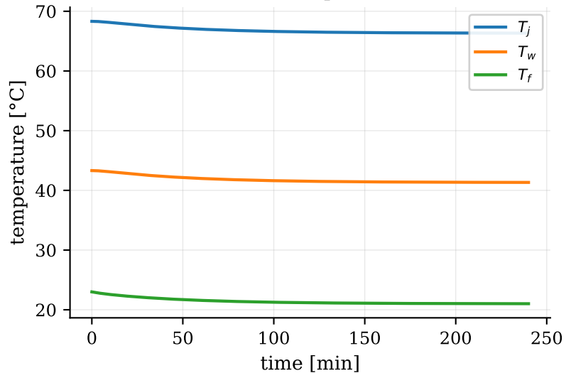
3-state, step Tin-2K
