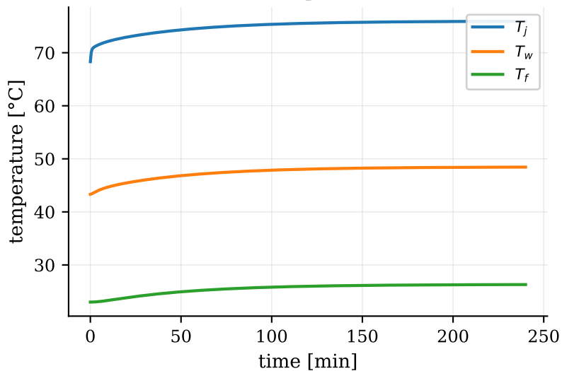
3-state, step QIT+10%
