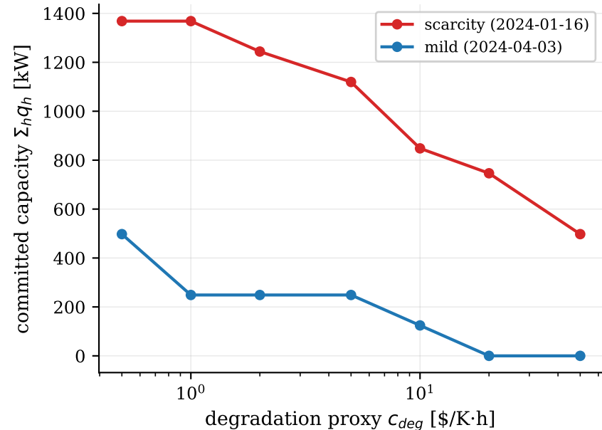
F3 — degradation-cost sensitivity of the certified S2 offer (d = 30 min, alibaba_jobaware trace)
