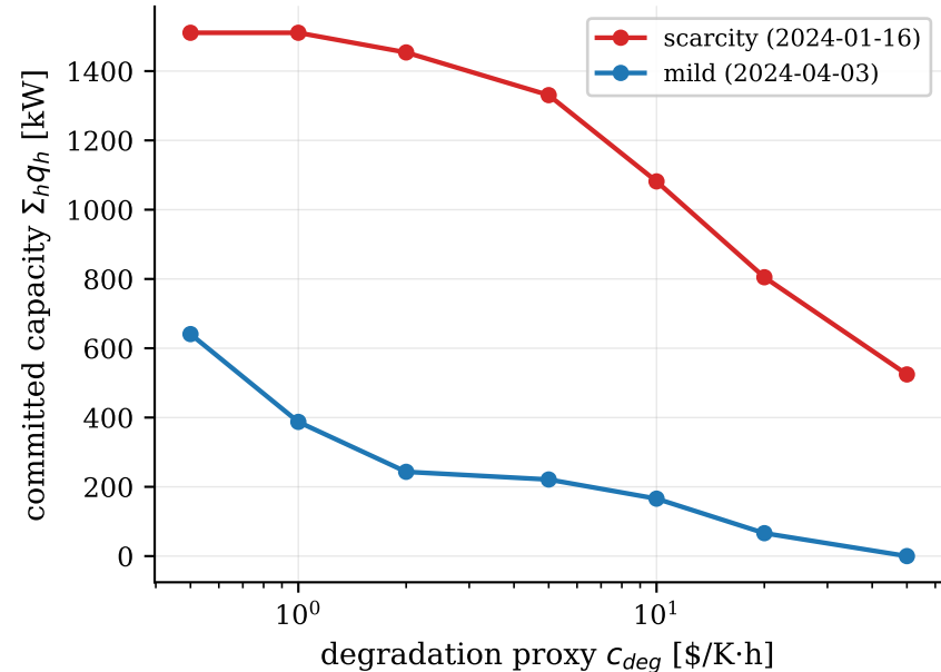
F3 — degradation-cost sensitivity of the certified S2 offer (d = 30 min, borg trace)
