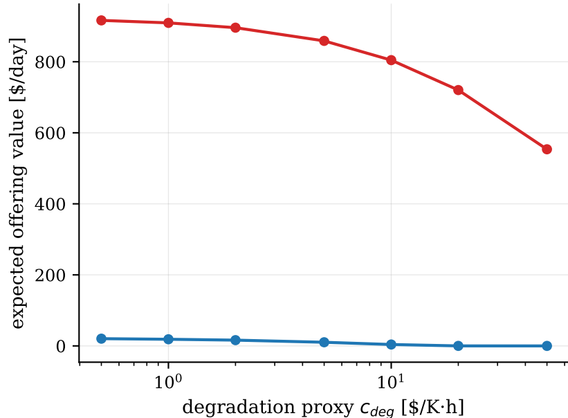
F3 — degradation-cost sensitivity of the certified S2 offer (d = 30 min, borg trace)
