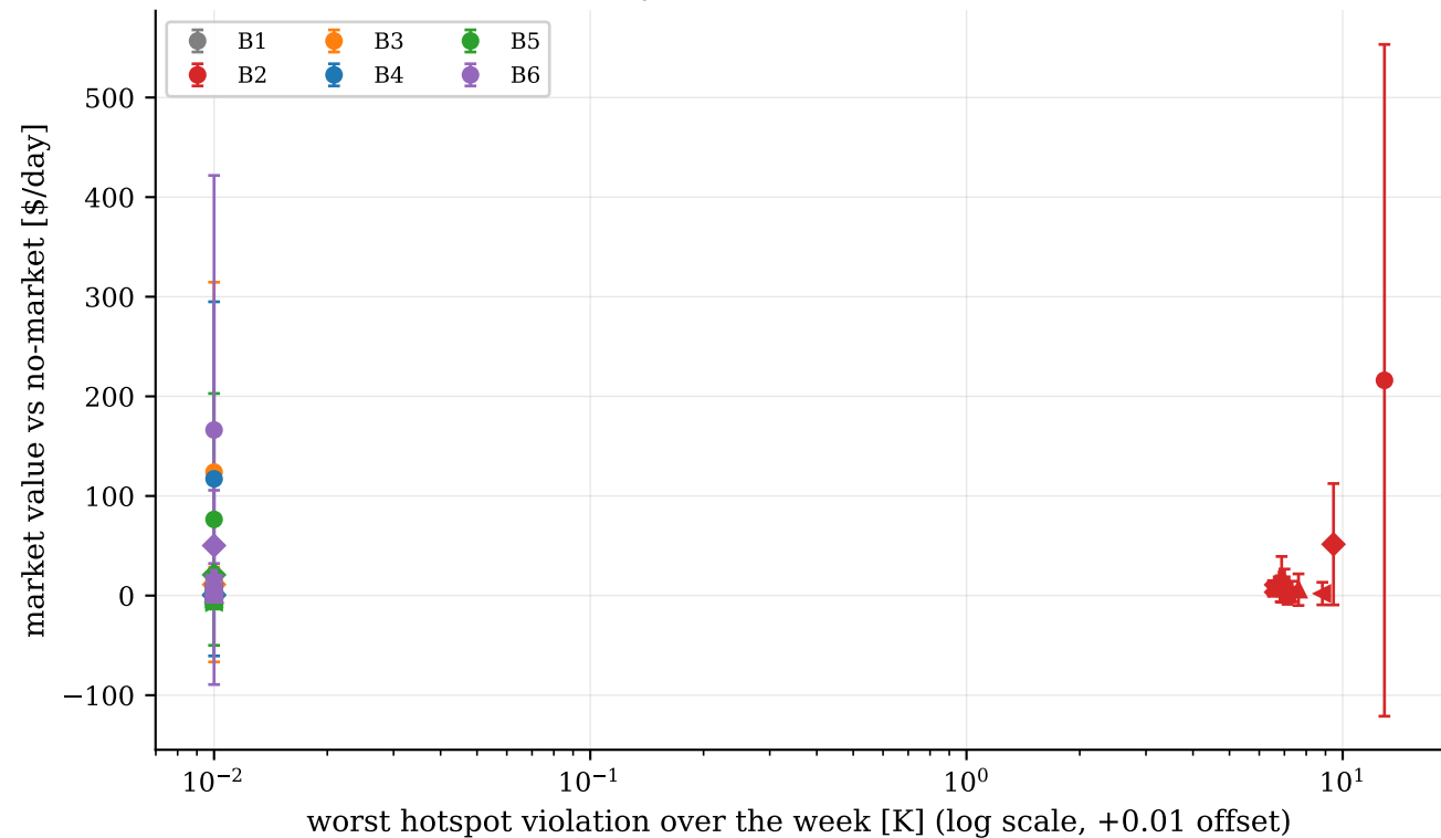
F2 — portfolio positioning, 10 real weeks \times 20 seeds (trainhall, S2 product) (markers by week; bars: \pm 1\sigma over seeds)
