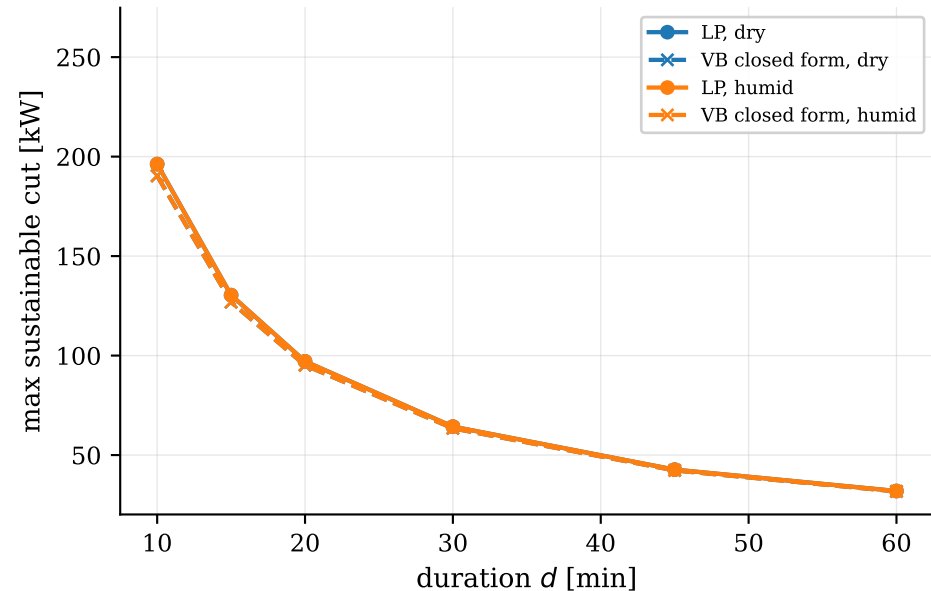
2-state (nominal start)
