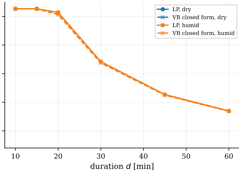
3-state (nominal start)
