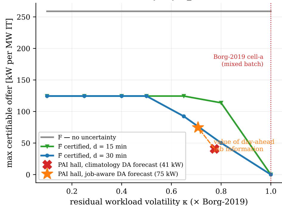
(a) the certification wall (dry day, T_{\text{dew}} = 12\text{ }^{\circ}\text{C} , \varepsilon = 0.3 )
