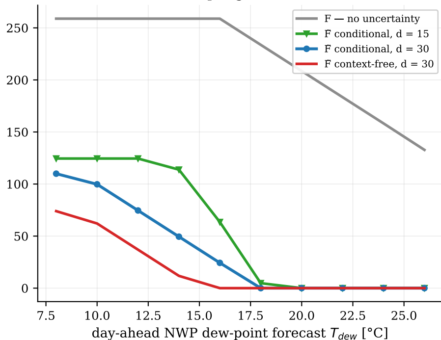
(b) weather coupling (PAI-workload hall)
