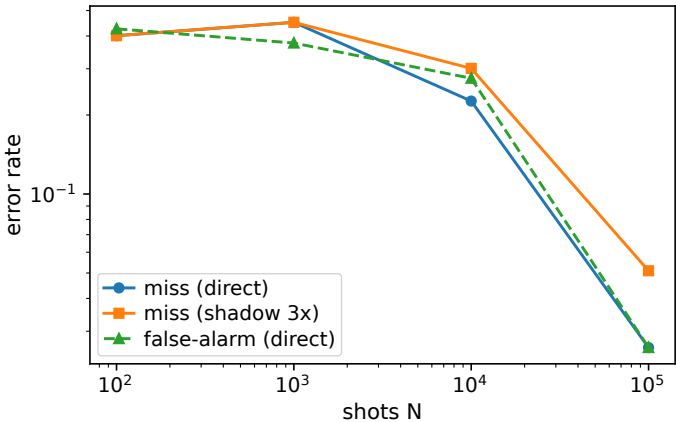
1q finite-shot detection
