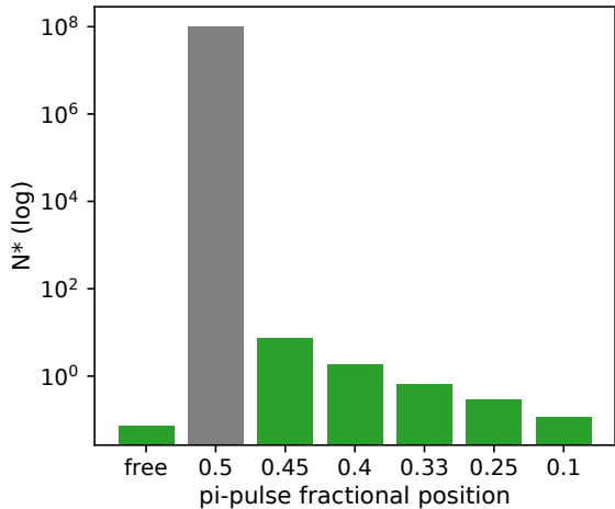
N^* for Z-detuning (gray = invisible)
