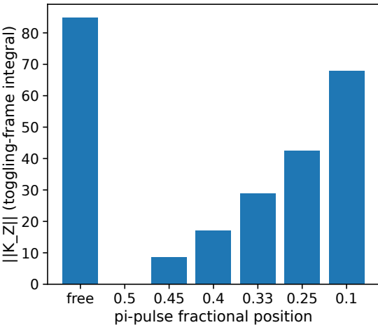
||K_Z|| vs pi-pulse position
