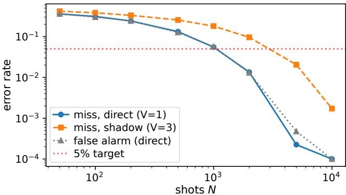
Detection error vs shots ( \gamma = 0.1 )
