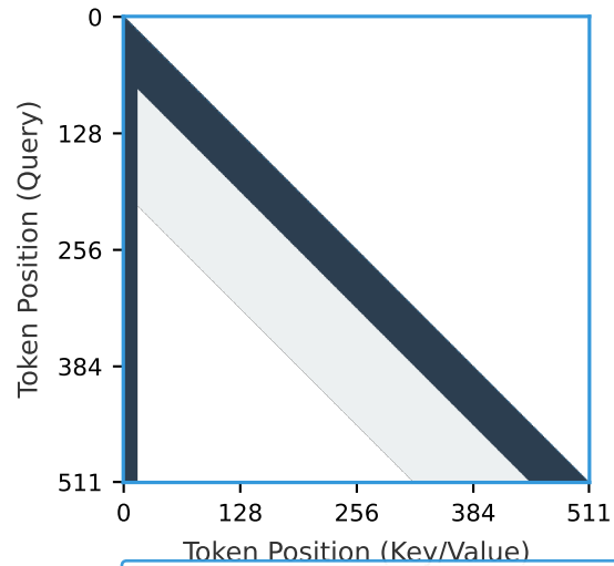
+Mixed-Precision
