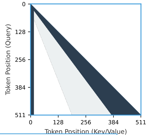
+Affine Window
