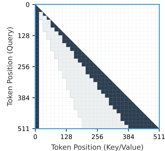
+Block-Aligned (B=16)
