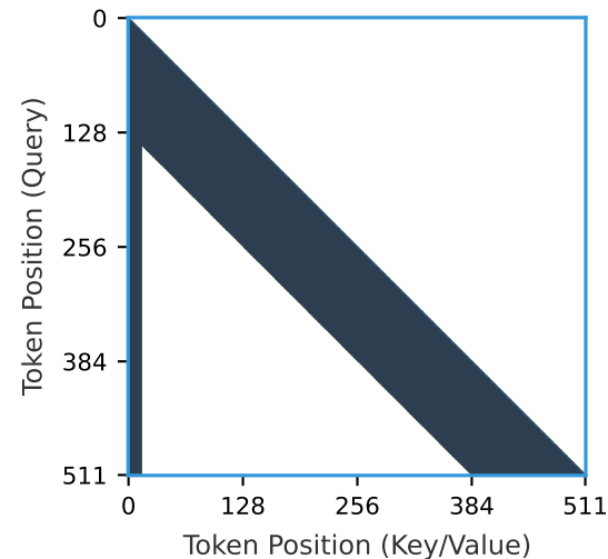
Causal Window Attention
