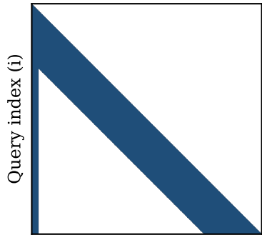
Causal Window
