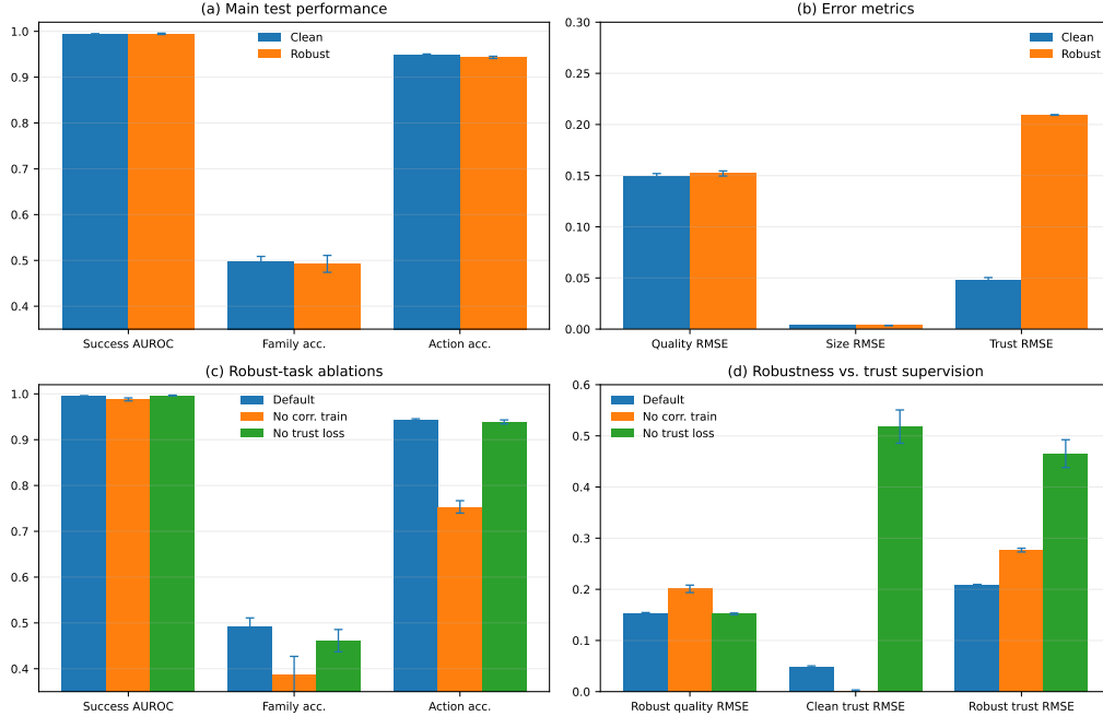
Figure 2: Five-seed robustness summary. Removing corruption-aware training substantially damages robust family accuracy, action accuracy, and quality estimation, whereas removing trust supervision mainly destroys the interpretability of trust estimates.
