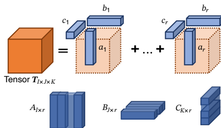
Figure 4: Illustration of Canonical Polyadic decomposition
