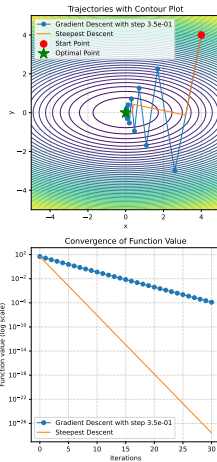
Figure 2: Steepest Descent
