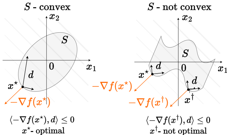
Figure 4: General first order local optimality condition
