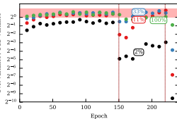
Figure 8: ResNet-110
