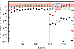
Figure 18: ResNet-110
