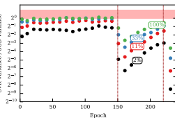
Figure 16: Small ResNet
