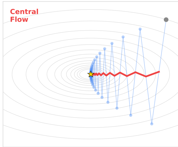
GD + Central Flow
