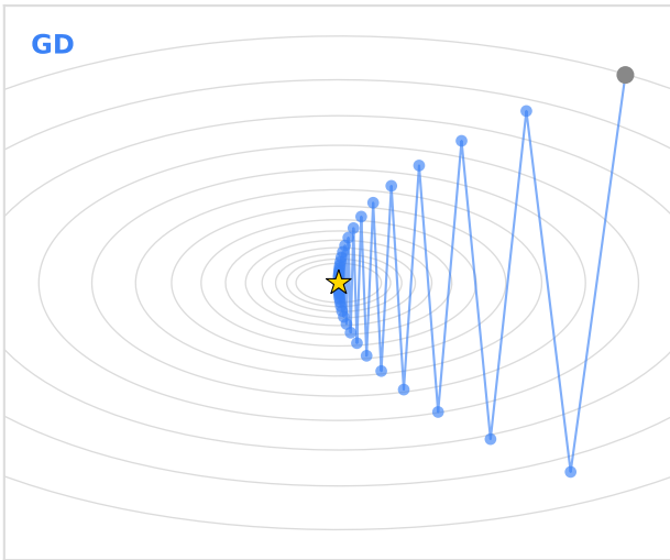
GD (edge of stability)
