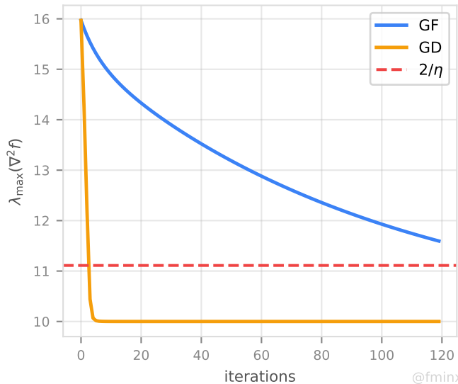
sharpness vs 2/\eta
