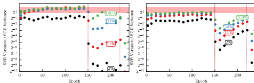
Figure 15: DenseNet
