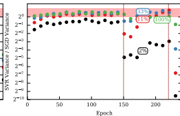
Figure 18: ResNet-110
