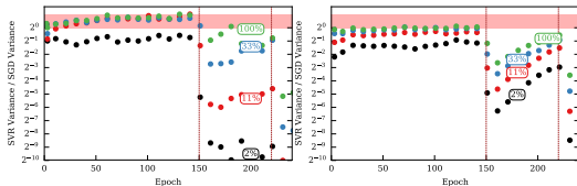
Figure 15: DenseNet
