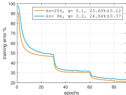
Figure 6: Без warmup
