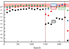
Figure 8: ResNet-110
