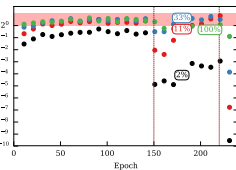
Figure 8: ResNet-110
