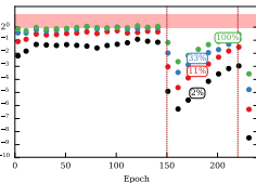
Figure 6: Small ResNet
