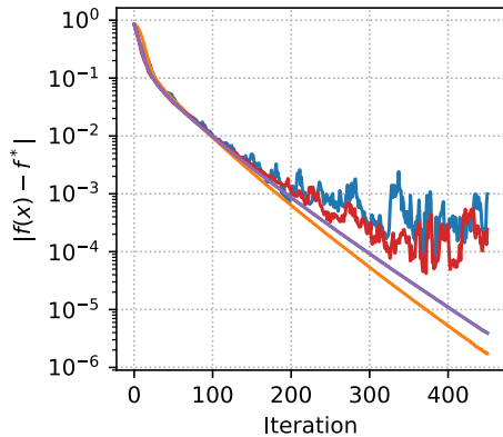
Strongly convex binary logistic regression. m=200 , n=10 , \mu=0.1 .
