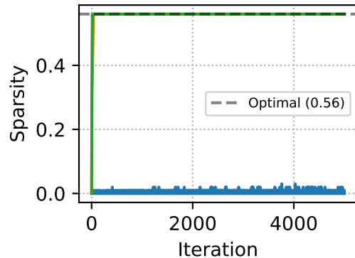
Sparsity of x_k
