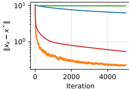
Distance to Optimal Solution
