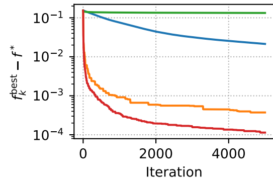
Function Gap
