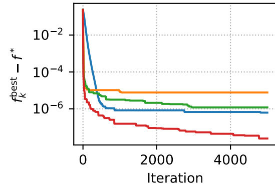
Function Gap
