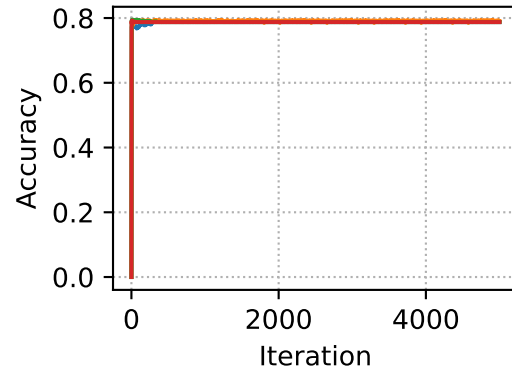
Train Accuracy
