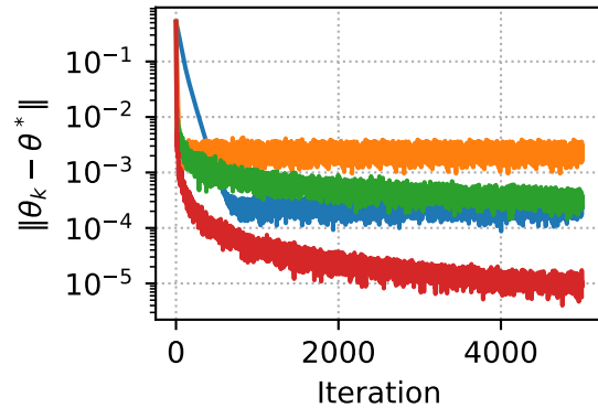
Distance to Optimal Solution
