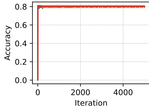
Test Accuracy
