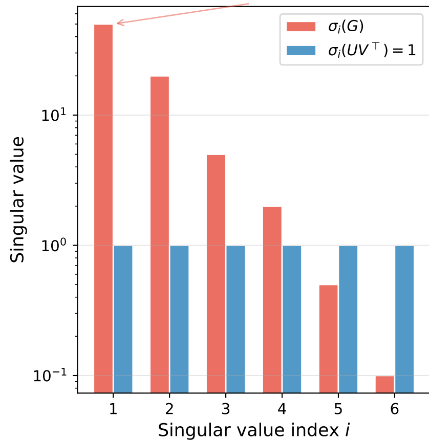
Gradient G vs Muon direction UV^\top
