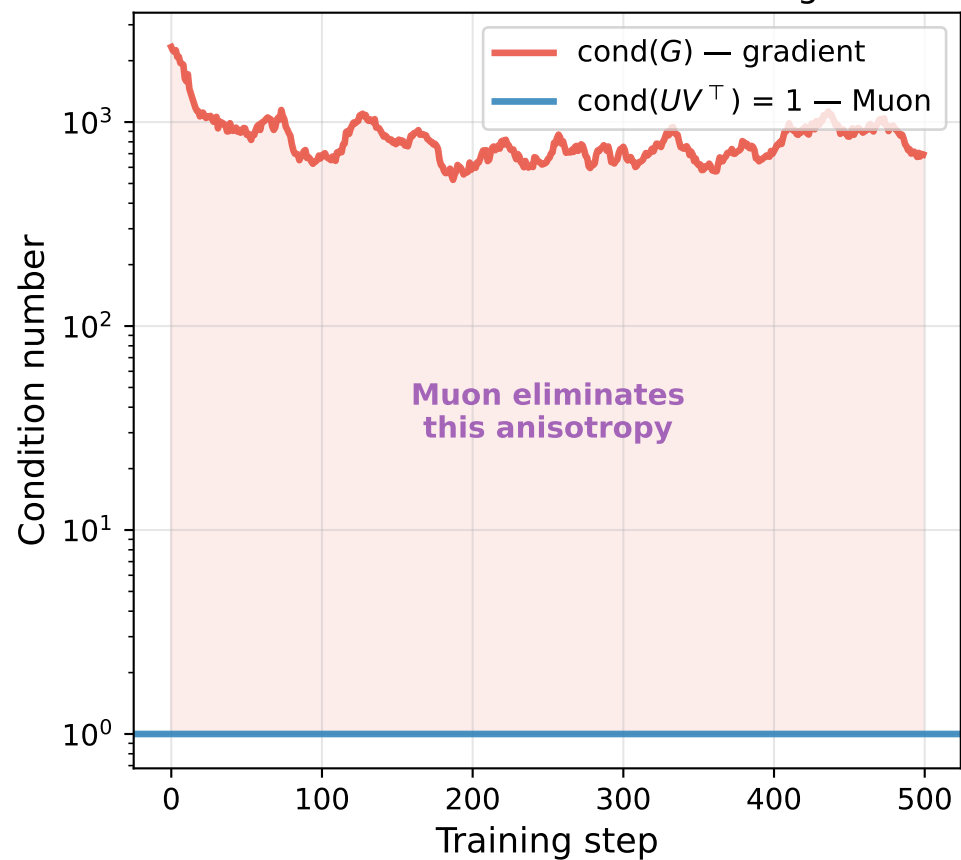
Gradient vs Muon: conditioning
