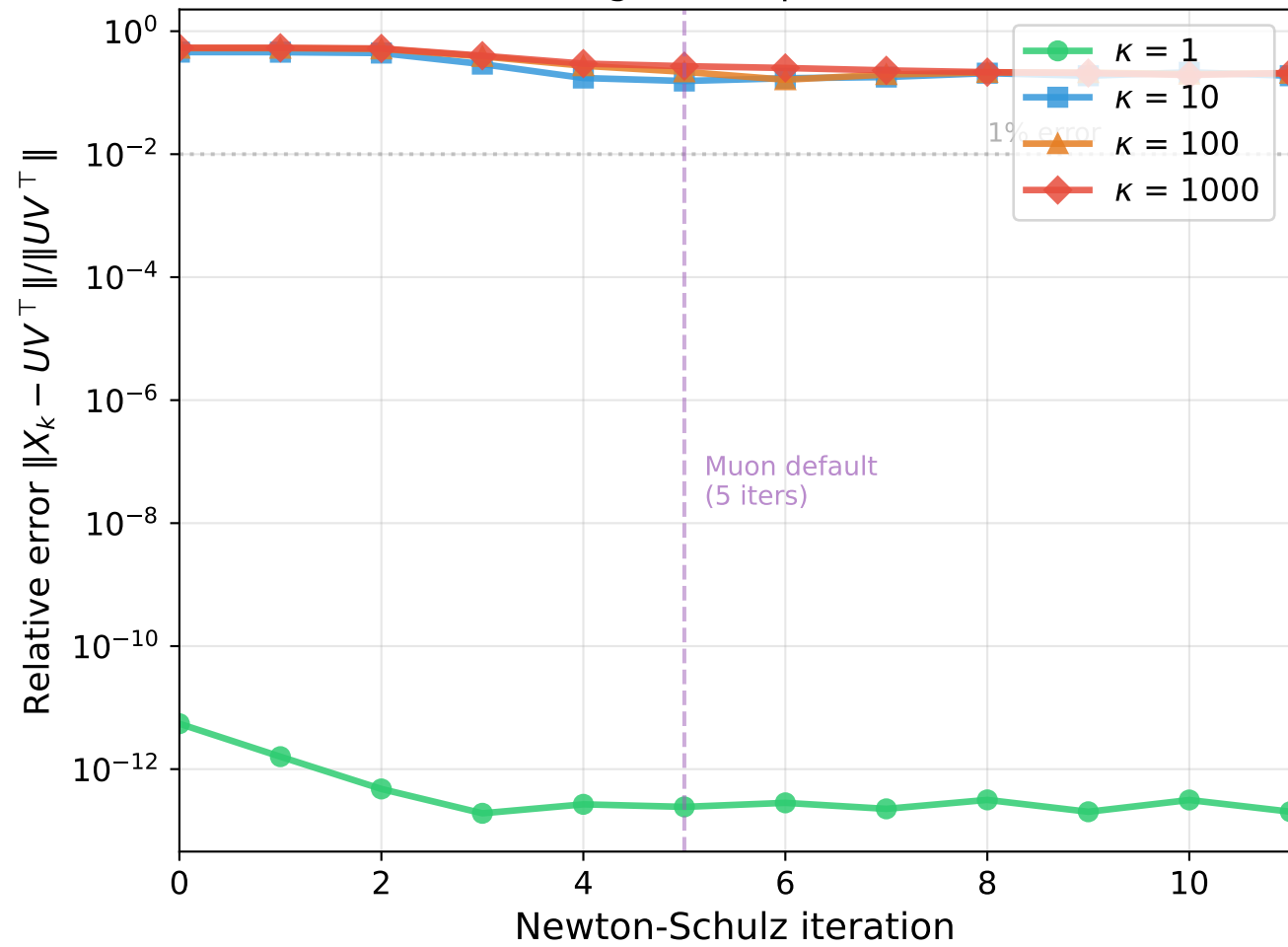
Convergence to polar factor
