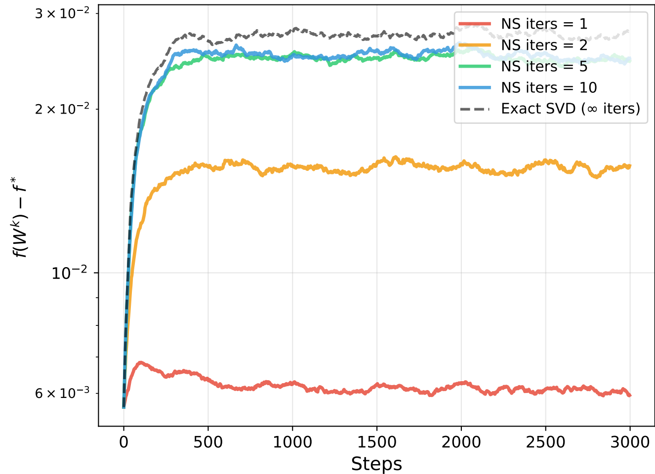
Muon: effect of Newton-Schulz iterations
