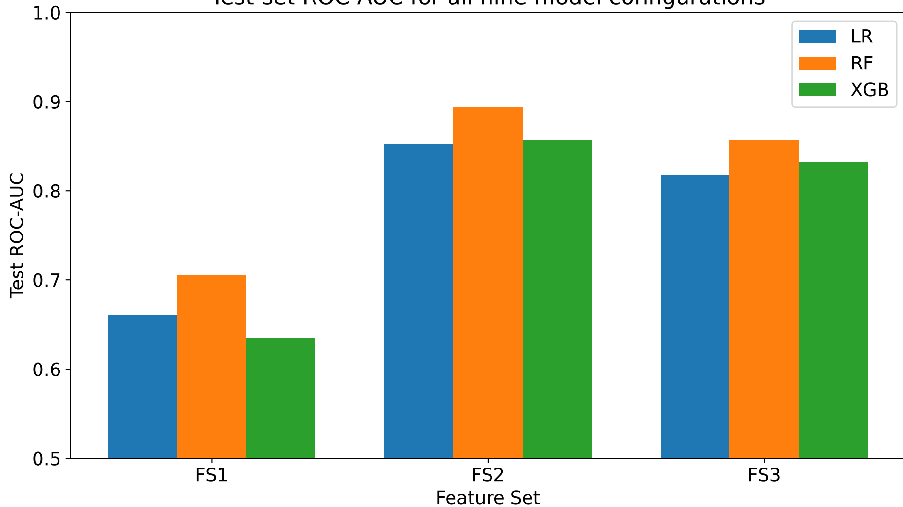
Test-set ROC-AUC for all nine model configurations
