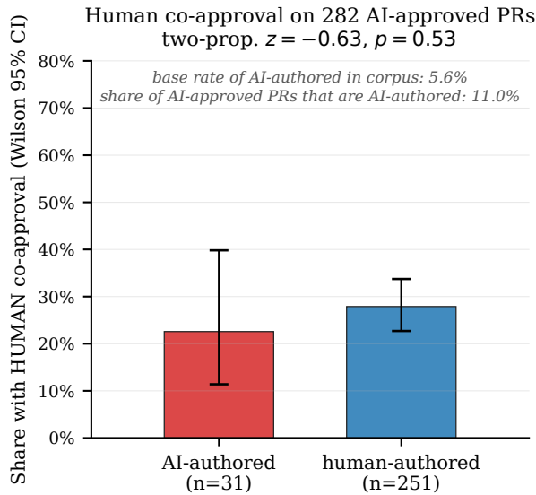
Figure 2. Human co-approval rate among the 282 PRs where an AI bot issued an APPROVED review. Red: AI-authored ( n=31 ). Blue: human-authored ( n=251 ). Point estimates differ by +5.3 percentage points (directionally consistent with AI reviewers approving AI code humans disagree with more often), but the two-proportion test is not significant ( p = 0.53 ) and the 95% CIs overlap — no statistically significant replication of the Laurito et al. (2025) single-turn AI-AI bias in this narrow slice. Error bars: Wilson 95% CIs. Not adjusted for code quality.
