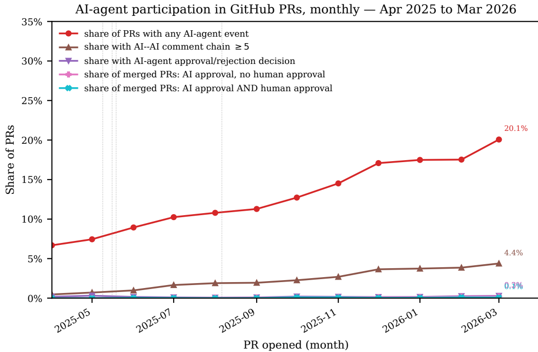
Figure 1. Monthly AI-agent participation in GitHub PRs across 3,000 popular repositories (Apr 2025–Mar 2026). Five series: share of PRs with any AI-agent event (RQ 1), share with an AI–AI comment chain of \geq 5 contiguous events (RQ 1), share with an AI-agent approval or rejection decision (RQ 2), share of merged PRs with an AI approval and no human approval (RQ 2), and share of merged PRs with both an AI and a human approval (RQ 2). Denominators vary (all PRs or merged-only). First- and last-month values are annotated on every line. Vertical dotted lines mark approximate public-availability dates of several coding and code-review agents (reader context, not a causal claim).
