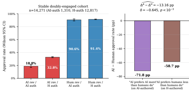
Figure 2. Within-PR AI-AI bias DiD on the 14,271 stable doubly-engaged PRs (AI bot reviewed and human reviewed, with no commitments between the AI’s verdict and the human’s review). Left: approval rates by reviewer-type ( \{AI, Human\} ) \times author-type ( \{AI, Human\} ); error bars are Wilson 95% CIs. Right: the two brackets in \hat{\Delta}^A - \hat{\Delta}^H — “AI prefers AI more than humans do” (-71.83 pp on AI-authored PRs) and “AI prefers humans less than humans do” (-58.67 pp on human-authored PRs). Their difference is the DiD: \hat{\Delta}^A - \hat{\Delta}^H = -13.16 pp (logit \delta = -0.645 , p < 10^{-3} ). Both brackets are negative because AI bots approve everything less than humans do; the bracket on AI-authored PRs is more negative, so the DiD is anti-self-preference.
