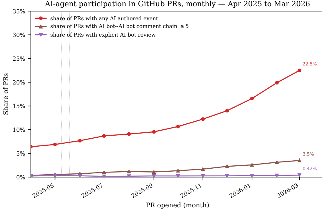
Figure 1. Monthly AI-system participation in GitHub PRs across 10,000 critical OS software repositories (Apr 2025–Mar 2026). Three series: share of PRs with any AI authored event — AI bot or AI powered (RQ 1), share of PRs with an AI–AI comment chain of \geq 5 contiguous AI bot events (RQ 1), and share of PRs with an explicit AI review (native AI bot APPROVED or CHANGES_REQUESTED review state; RQ 2). First- and last-month values are annotated on every line. Vertical dotted lines mark approximate public-availability dates of several coding and code-review agents (reader context, not a causal claim).
