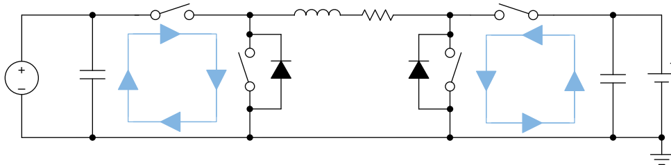
Figure 86. Buck-Boost Converter High Frequency Current Path
