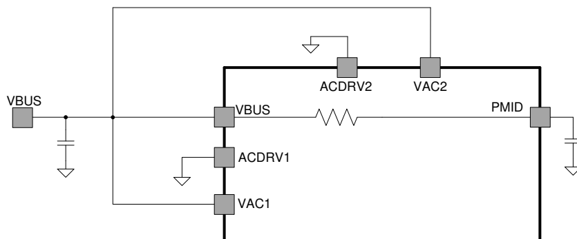
Figure 1. Single Input Connected to VBUS Directly Without ACFET-RBFET
