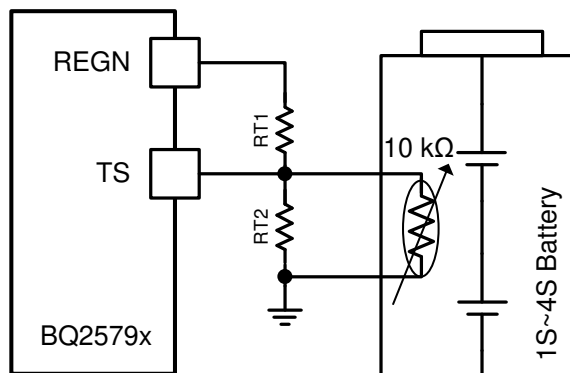
Figure 13. TS Resistor Network
