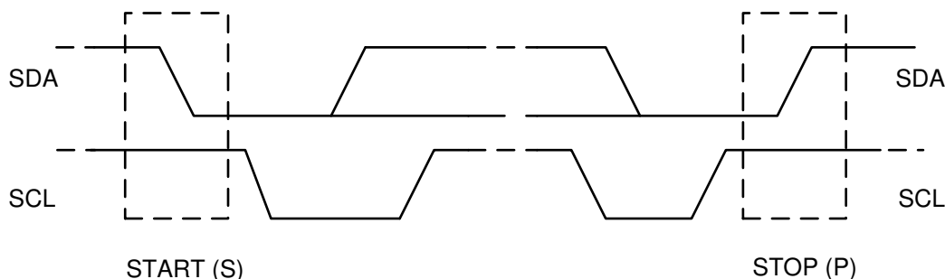
Figure 18. START and STOP Conditions on the I 2 C Bus
