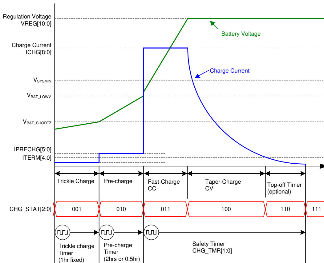
Figure 11. Battery Charging Profile
