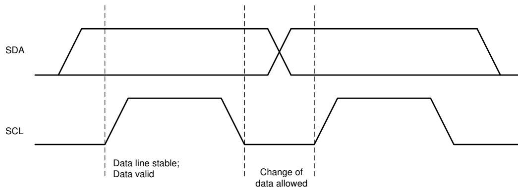
Figure 17. Bit Transfers on the I 2 C Bus
