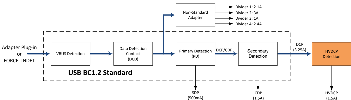
Figure 6. D+/D- Detection Flow
