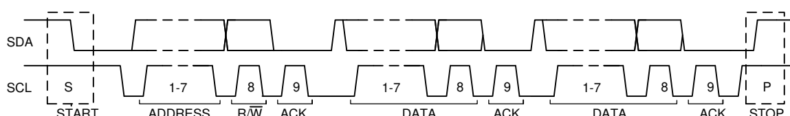
Figure 21. Complete Data Transfer on the I 2 C Bus
