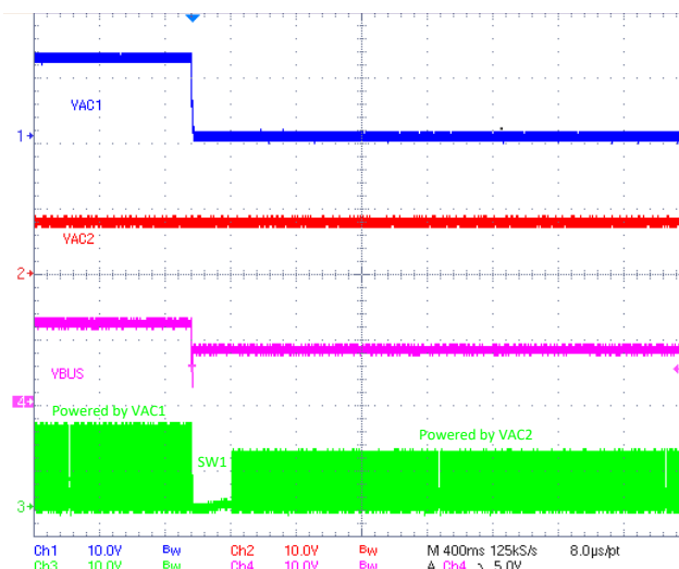
Figure 4. Input Source Auto Transition from VAC1 to VAC2 when VAC1 is Gone
