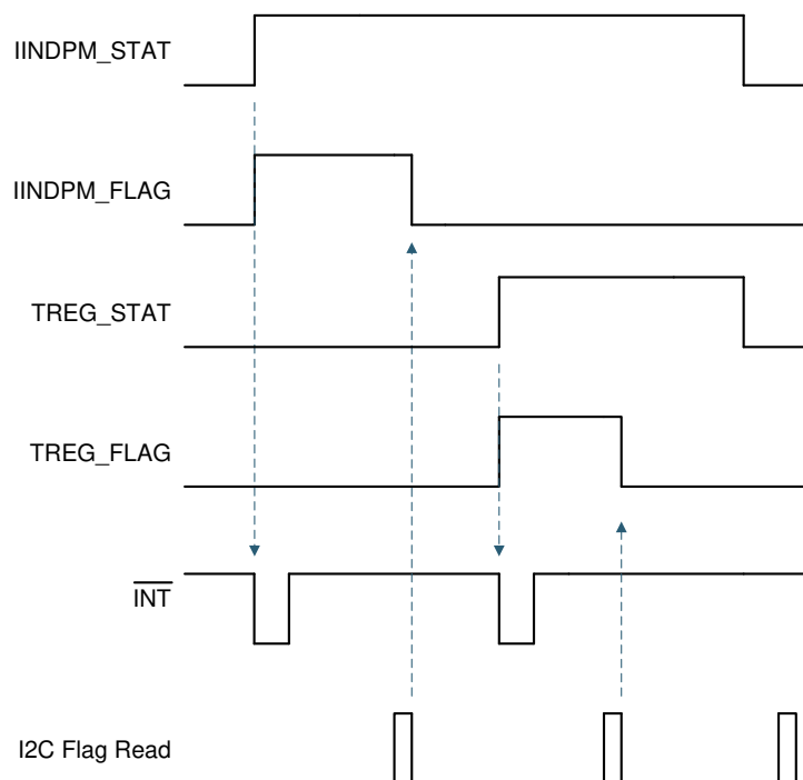
Figure 15. \overline{\text{INT}} Generation Behavior Example
