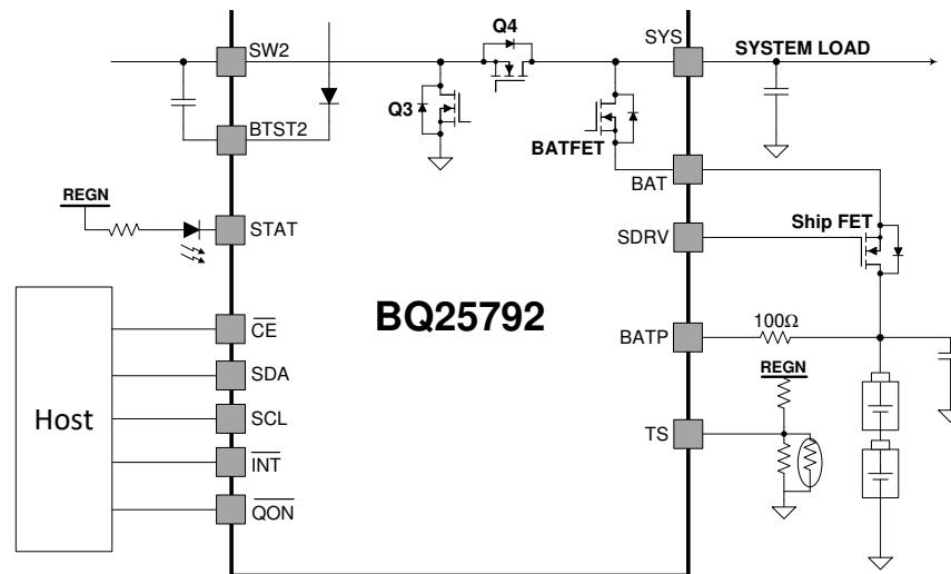
Figure 16. The Application Diagram for the External Ship FET
