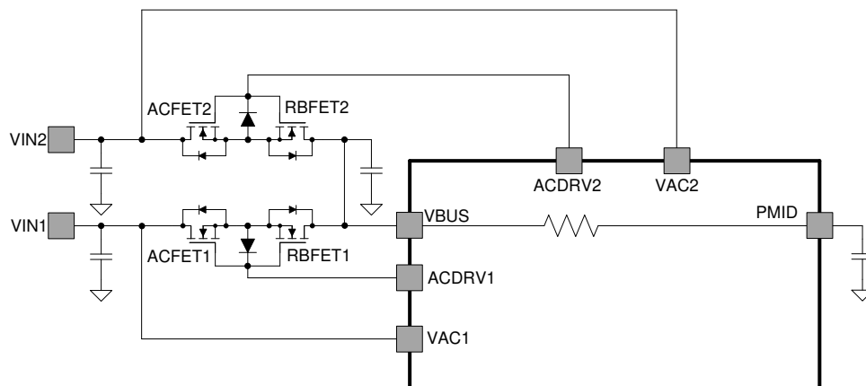
Figure 3. Two ACFETs-RBFETs Structure Supporting One Input at VAC1 and One Input at VAC2
