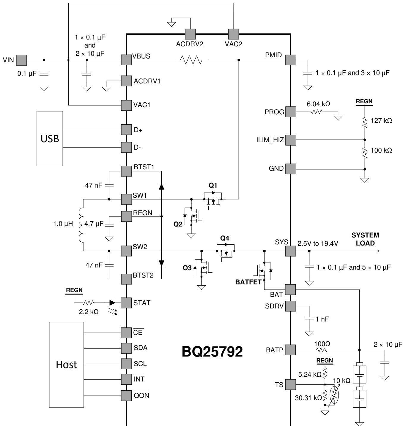
Figure 85. BQ25792 Application Diagram with Single Input Source and No Ship FET
