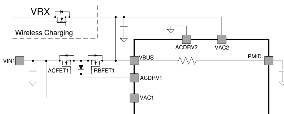
Figure 2. One ACFET-RBFET Structure Supporting One Input at VAC1 and/or One Input at VBUS
