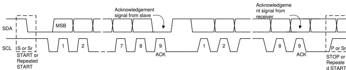
Figure 19. Data Transfer on the I 2 C Bus
