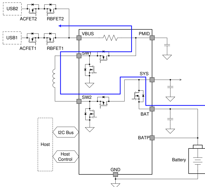
Figure 7. The Simplified Application Diagram for the OTG Mode Operation
