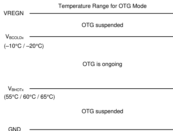
Figure 14. TS Pin Thermistor Sense Threshold in OTG Mode
