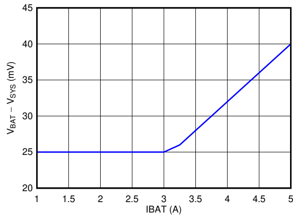
Figure 9. BATFET I-V Curve
