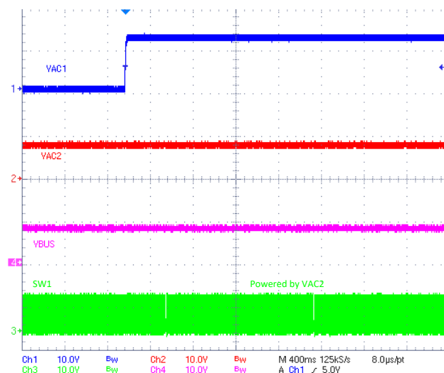
Figure 5. VAC1 Re-Plugged in When VAC2 Connected as the Charger Input
