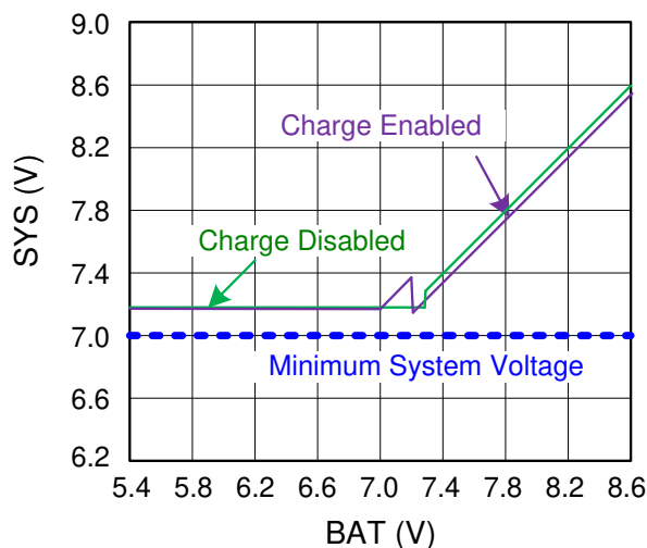
Figure 8. Typical System Voltage vs Battery Voltage for a 2S Battery Configuration
