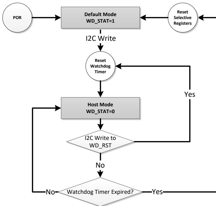
Figure 26. Watchdog Timer Flow Chart
