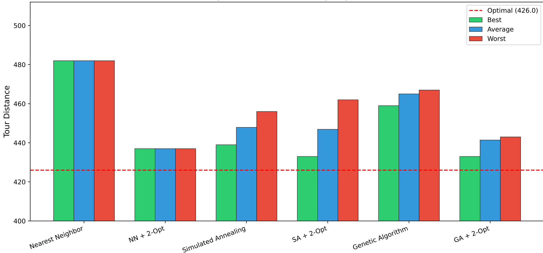
Best / Average / Worst Distance by Algorithm (eil51)
