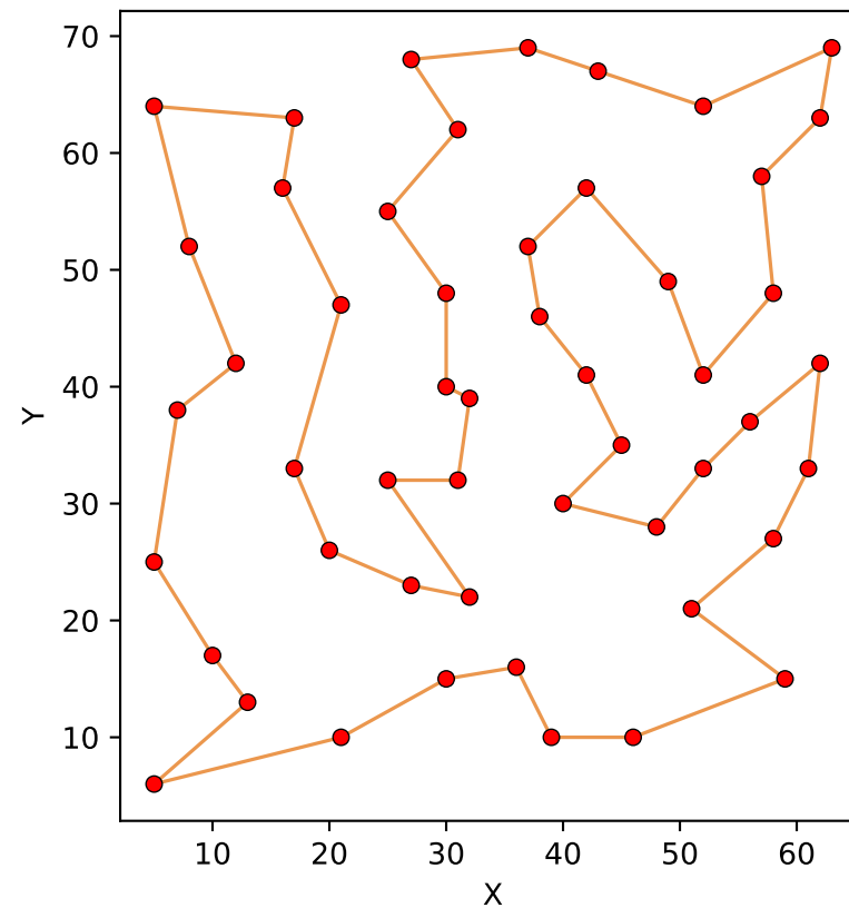
Genetic Algorithm Distance: 467.00
