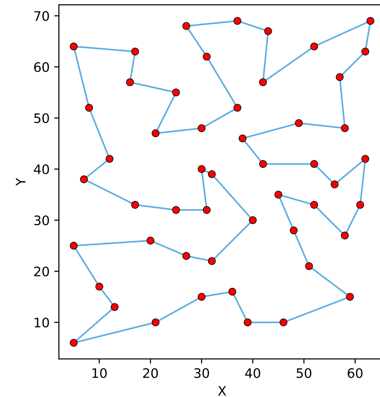
GA + 2-Opt Distance: 443.00
