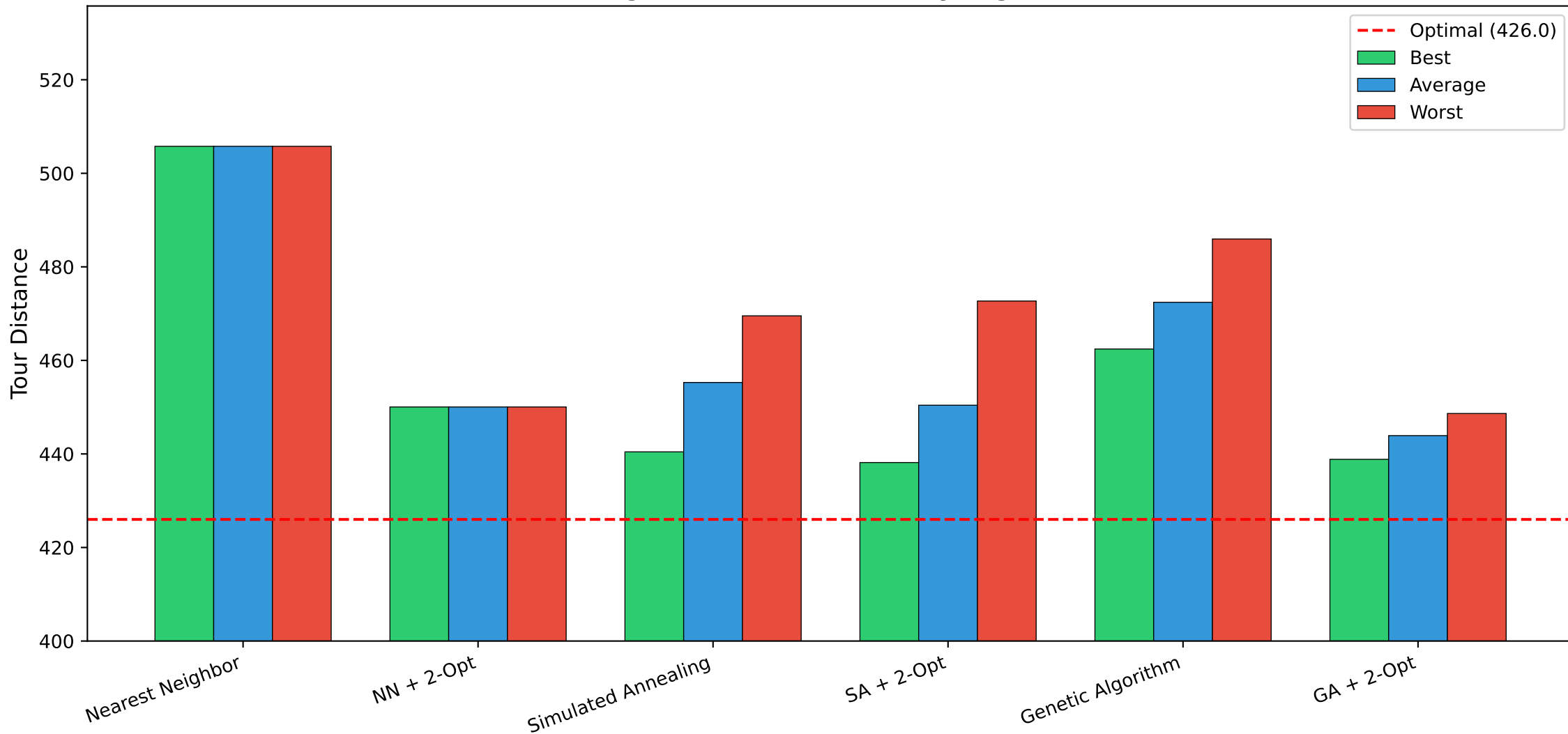
Best / Average / Worst Distance by Algorithm (eil51)
