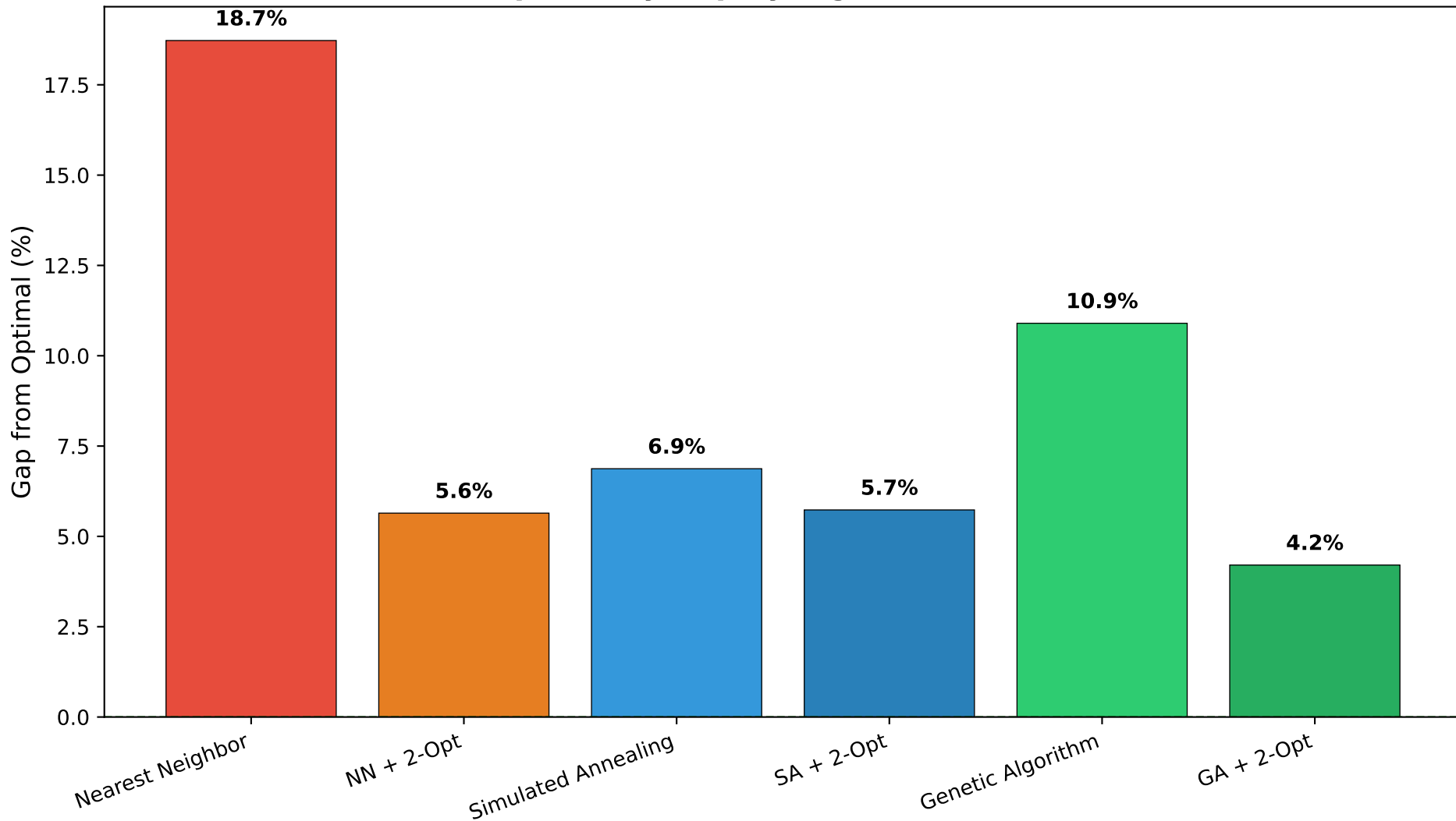
Optimality Gap by Algorithm (eil51)
