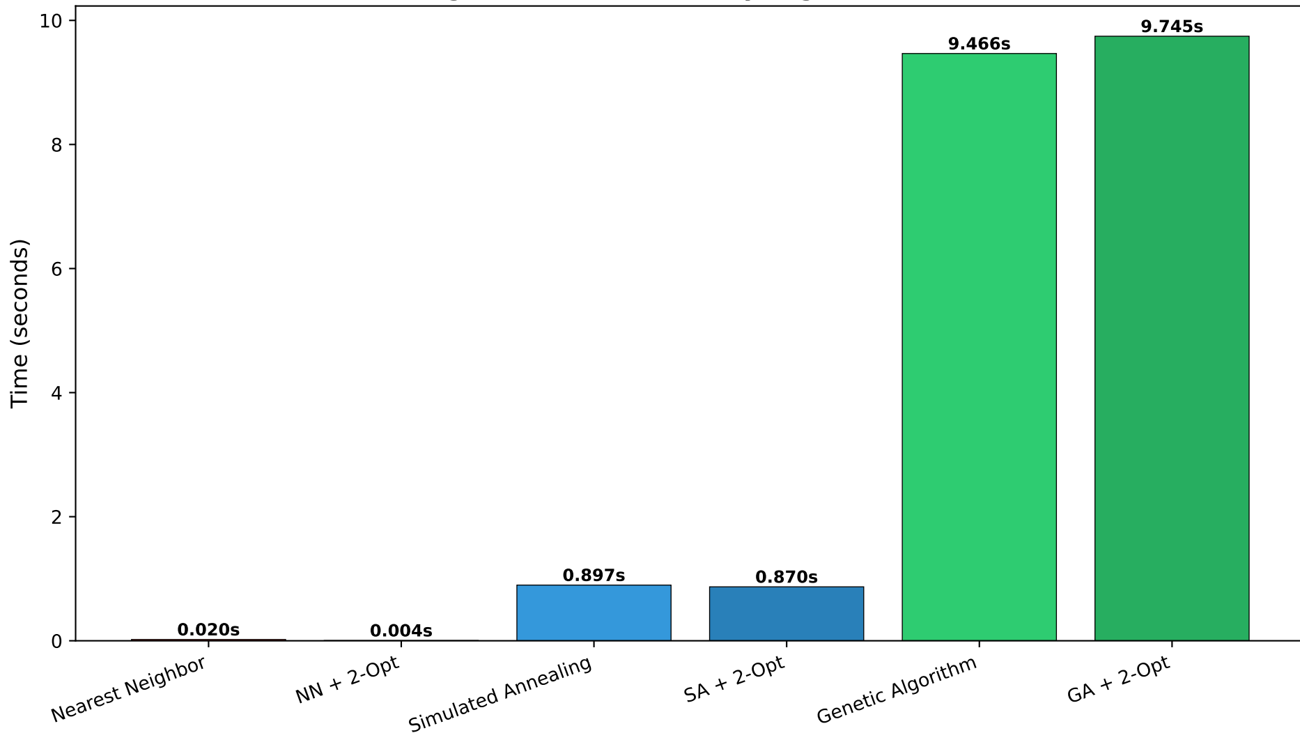
Average Execution Time by Algorithm (eil51)
