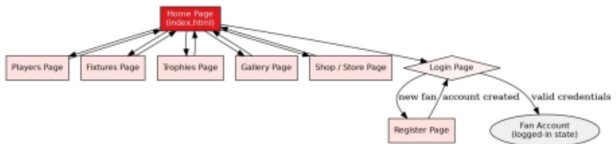
Figure 2: Navigation Flowchart (UI Design)
