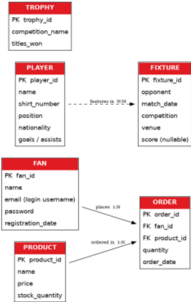
Figure 3: Entity Relationship Diagram (ERD)
