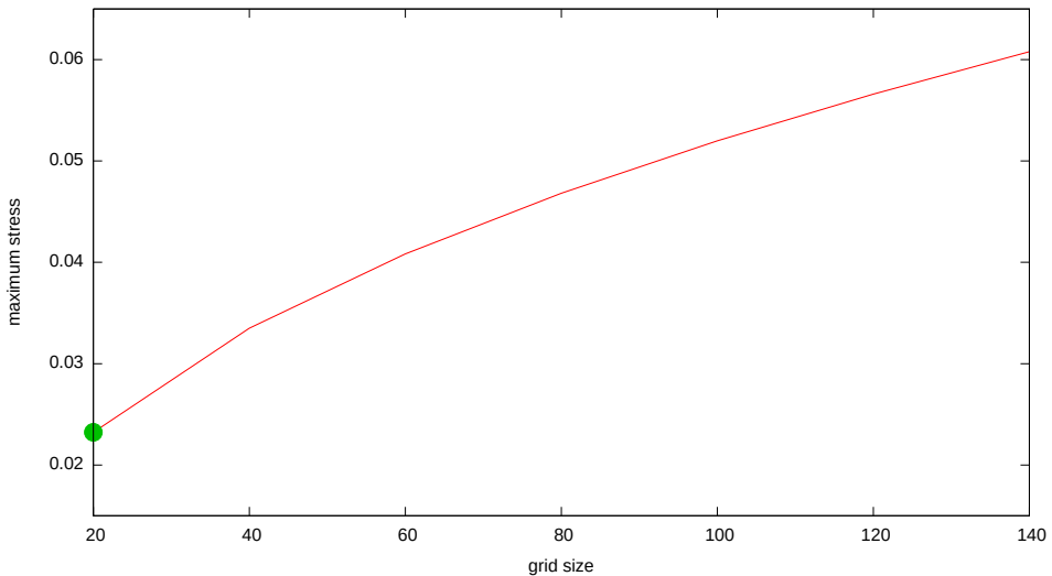
pie_90 Maximum Stress Under Refinement
